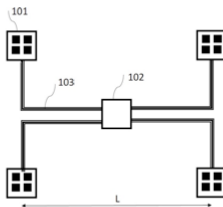
mm-wave arrays with two or more subarray modules (101), a central processing unit (102) and mm-wave/sub-mm-wave low-loss interconnects (103)
