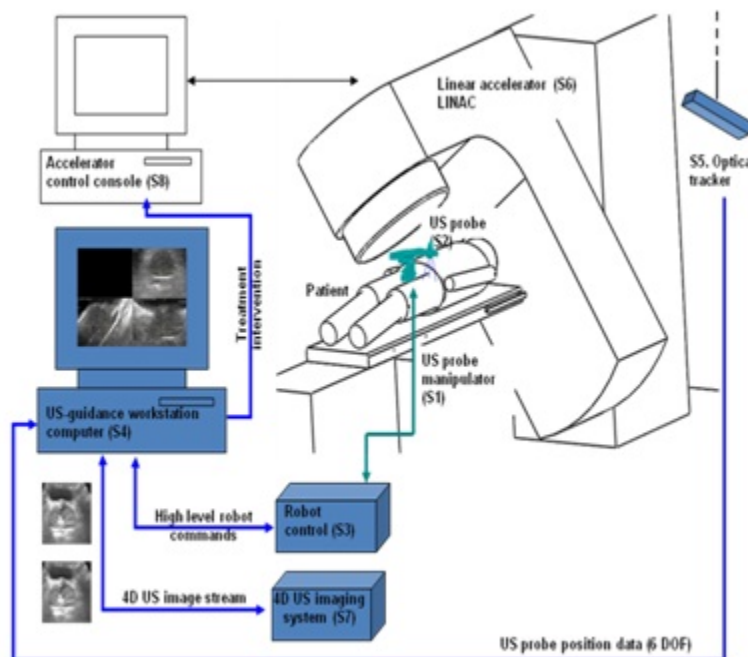
Figure 1 - Robotic ultrasound image guidance system in radiation therapy (Image courtesy the Hristov Lab and Salisbury Robotics Lab)
