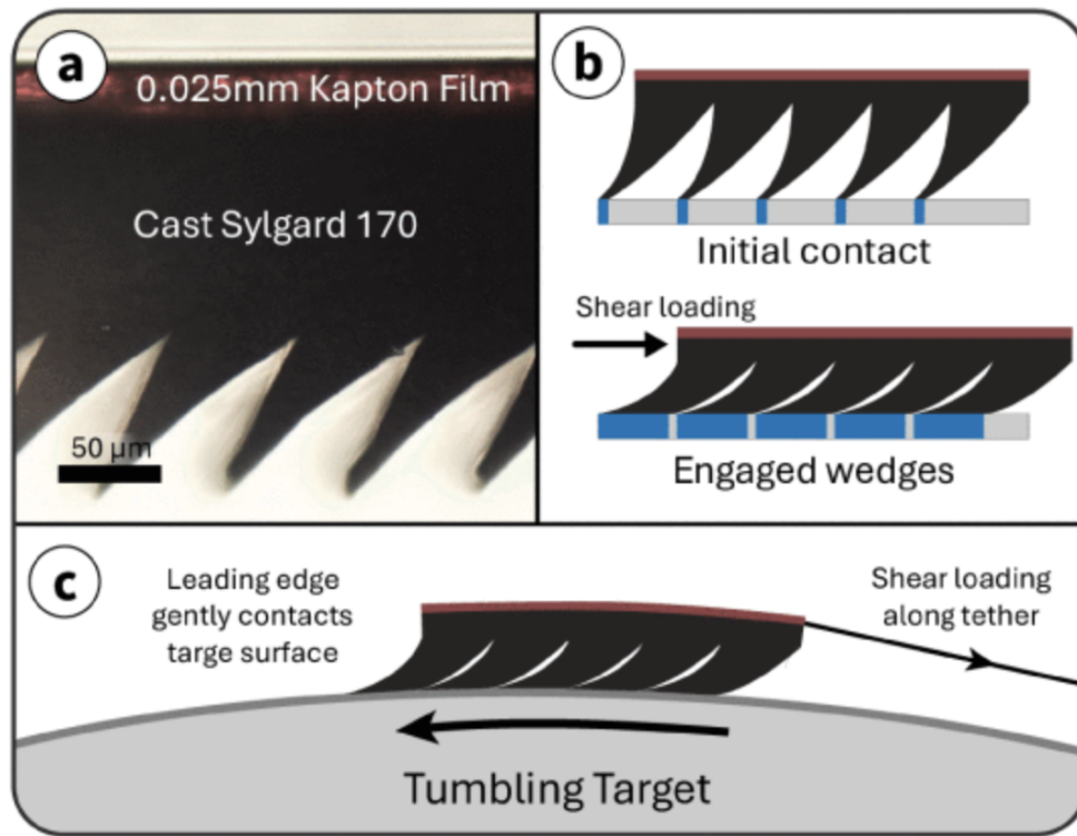
Figure 2 Gecko Lasso Anisotropic adhesive geometry (a), engagement details (b), and shear loading (c)
